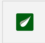
Thymeleaf
