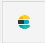
Elastic Search
