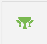
Grails
