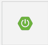
Spring Boot
